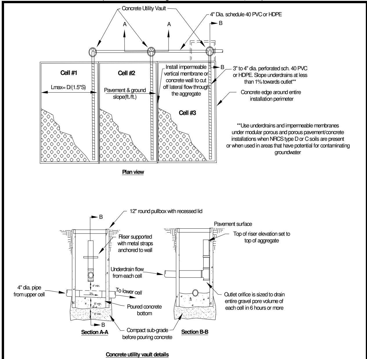
Figure 4-53. Schematic of an Underdrain System
