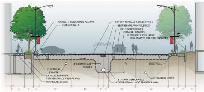
Street section
